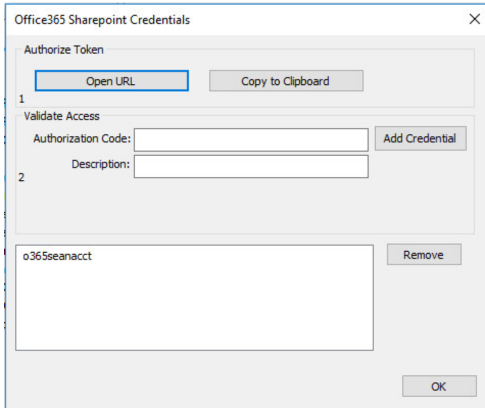
Credentials Dialog
