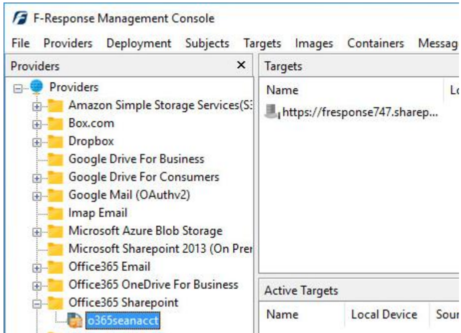
Listing Targets
